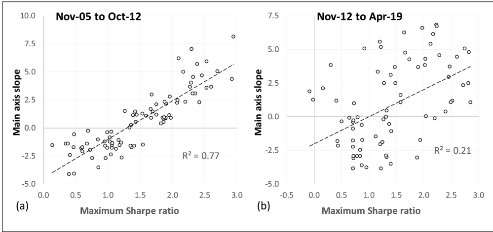
FIGURE 5 S_{MA} regressed on the tangent portfolio's maximum Sharpe ratios for the period (a) Nov-05 to Oct-12 and (b) Nov-12 to Apr-19
