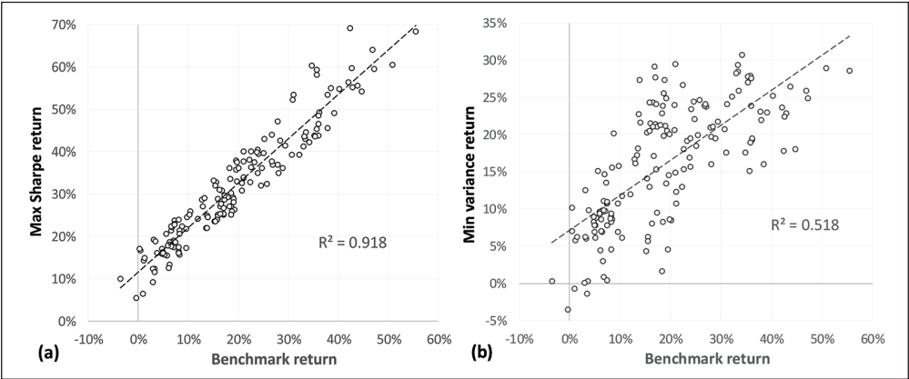
FIGURE 10 Regression of (a) monthly maximum Sharpe ratio portfolio returns and (b) monthly minimum variance portfolio returns on monthly benchmark portfolio returns
