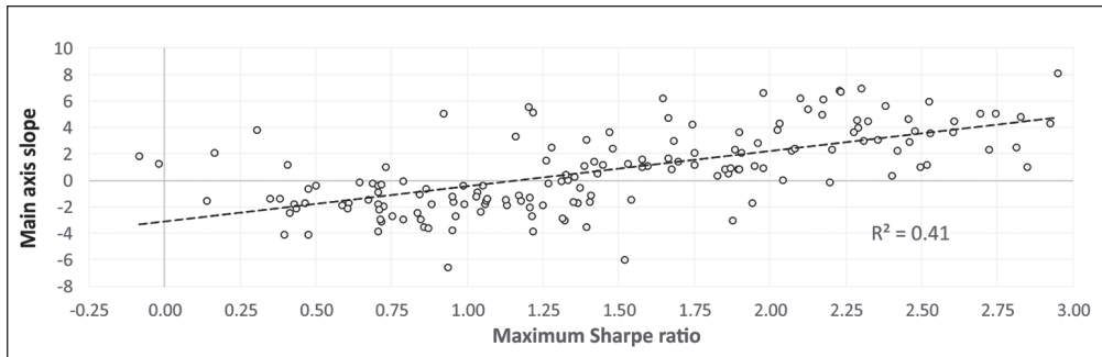
FIGURE 4 S_{MA} regressed on the tangent portfolio's maximum Sharpe ratios
